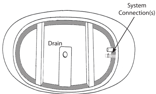
Open Bottom
