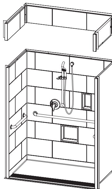
Back wall left fixture placement configuration shown with optional soap dish
