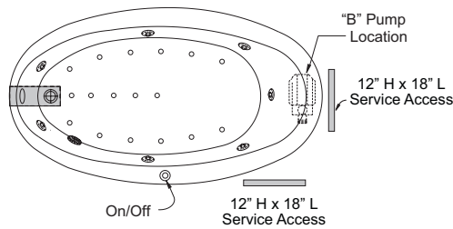
ALTERNATE PUMP LOCATION
