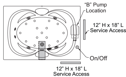
ALTERNATE PUMP LOCATION
