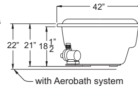
END VIEW
