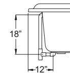
DRAIN / OVERFLOW
